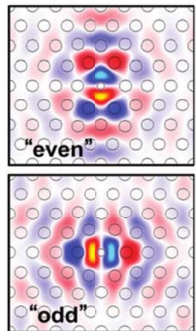
Fig. II Resonating optical modes in a photonic crystal cavity
