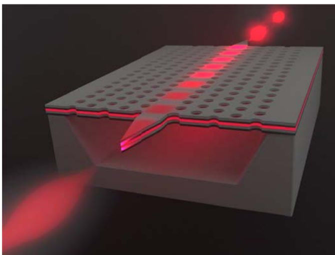
Fig. II Artistic illustration of a photonic crystal waveguide that amplifies optical pulses
