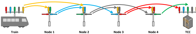
Figure 8.12: Separate frequency for train-to-trackside communication combined with extended frequency separation
