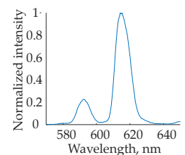
Figure 4.1: The emission spectrum of europium chelate, measured at Radiometer Turku. The emission peak is at 615 nm.
