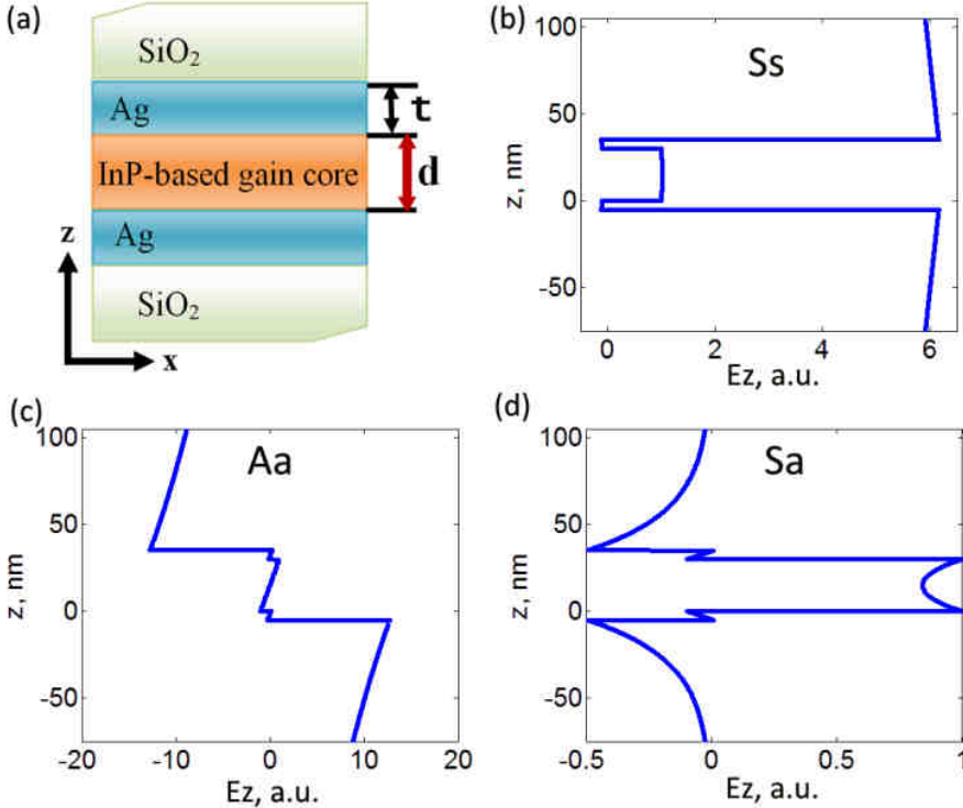
Fig. 5.1. (a) Finite-thickness MSM waveguide. (b), (c), (d) E_z field profile in the waveguide with d = 30 nm and t = 5 nm for Ss, Aa and Sa modes, respectively. The field is normalized such that E_z = 1 a.u. at the interface between gain core and metal layer.
