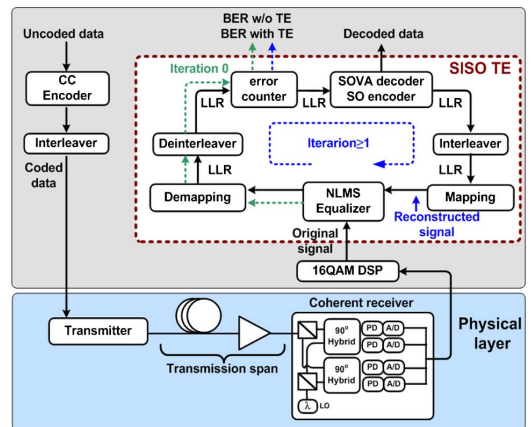
Fig. 1. Pre-encoding and receiver structure of the SISO turbo equalizer algorithm. CC, convolutional code; LO, local oscillator; PD, photodiode; A/D, analog-to-digital converter; DSP, digital signal processing; NLMS, normalized least mean square; LLR, log-likelihood ratio; SOVA, soft-output Viterbi algorithm; SO, soft output; SISO, soft-input soft-output; TE, turbo equalization.
