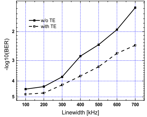
Fig. 6. BER as a function of transmitter and local oscillator laser linewidth for back-to-back with fix OSNR value of 25 dB.
