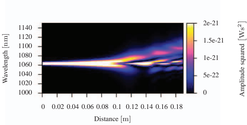
(a) The spectral evolution is shown as a contour plot of wavelength and longitudinal position in the fibre. The soliton is observed to SSFS to the transfer wavelength of 1100 nm.
