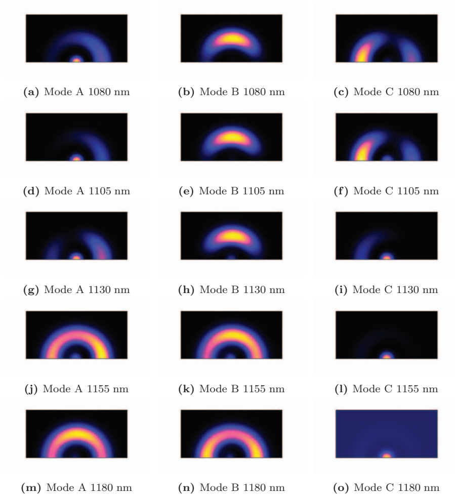
Figure 7.16: The flow of intensity in the longitudinal direction for the modes A, B, and C in Fig. 7.15 at different wavelengths. The dimensions of the intensity plots are from -10 \mu\text{m} to 10 \mu\text{m} in the x -direction and from 0 \mu\text{m} to 10 \mu\text{m} in the y -direction. The bright colours represent areas of high intensity, whereas the darker represent areas of low intensity on a linear scale.
