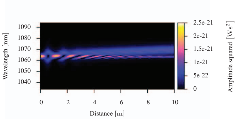
(a) Simulation using the implementation of the GNLSE with the fourth root method of the effective area.
