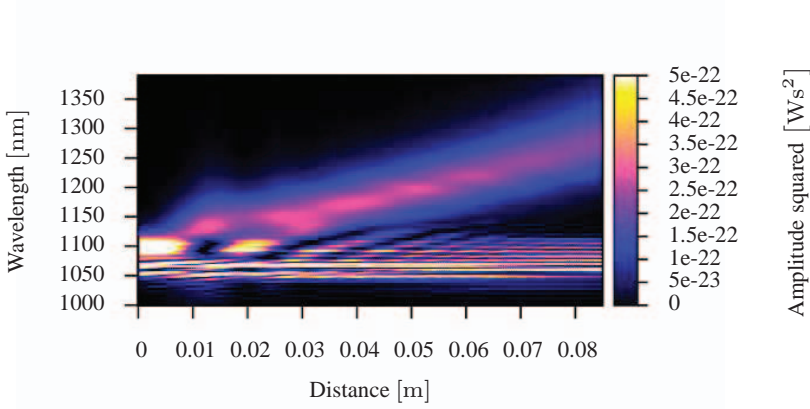
(a) The spectral evolution is shown as a contour plot of wavelength and longitudinal position in the fibre. The soliton is observed to SSFS to a wavelength of 1280 nm.
