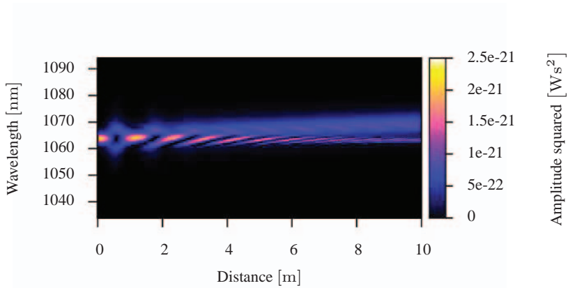
(b) Simulation using the implementation of the TFD-GNLSE with the correct dispersion of the transverse field distribution.
