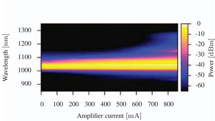
(a) The spectral evolution is shown as a contour plot of wavelength and current to the third amplifier pump in the fibre.
