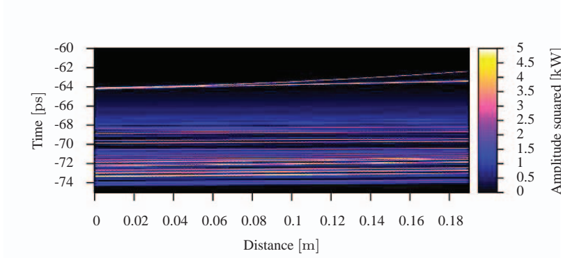
(a) The temporal evolution is shown as a contour plot of time and longitudinal position in the fibre.
