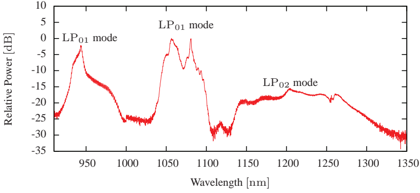
(a) The measured output spectrum.
