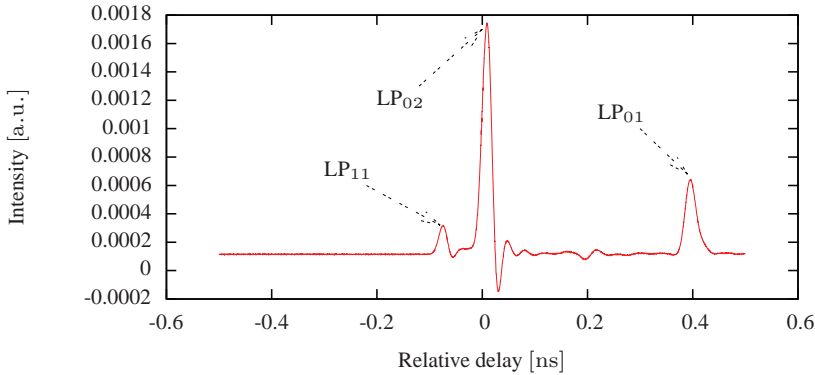
Figure 4.14: An example of the recorded temporal trace at a wavelength of 1064 nm.
