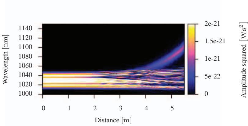
(a) The spectral evolution is shown as a contour plot of wavelength and longitudinal position in the fibre. The soliton is observed to SSFS to the transfer wavelength of 1100 nm. To compensate for the chirped before forming a soliton pulse the length of the LSF is longer than for the case with an unchirped femtosecond pulse.
