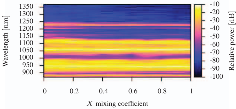
(b) Calculated LP_{0,1} output spectrum with the TFD-GNLSE.
