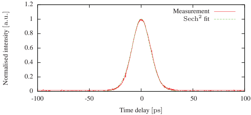
Figure 5.9: Intensity autocorrelation for the ANDi PM laser.
