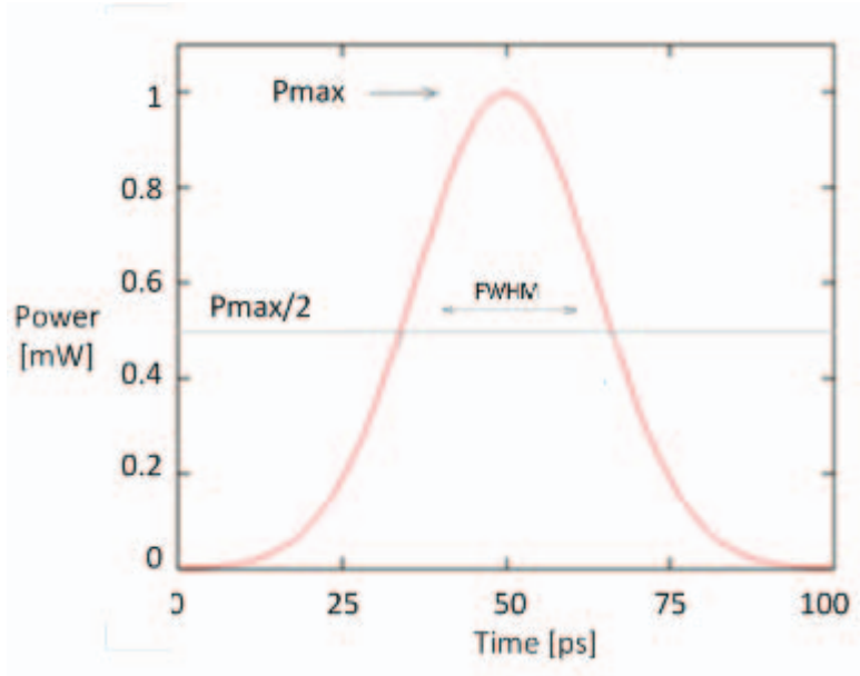
Figure 3-12: FWHM definition
