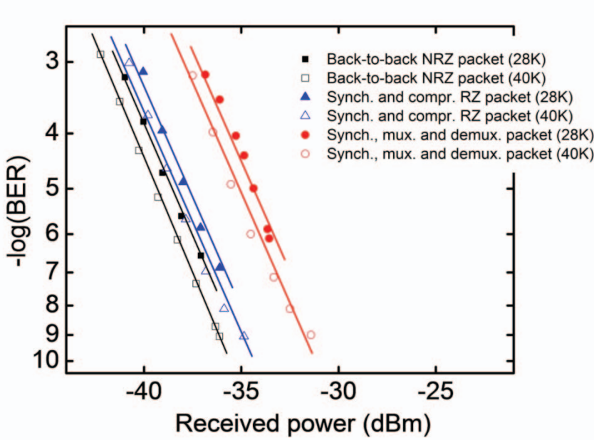
Figure 5-8: BER measurements
