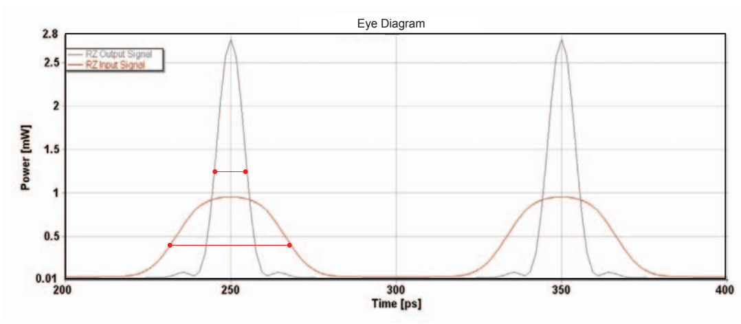
Figure 3-13: FWHM: eye-diagram for output RZ signal ( \Delta t = 0 )
