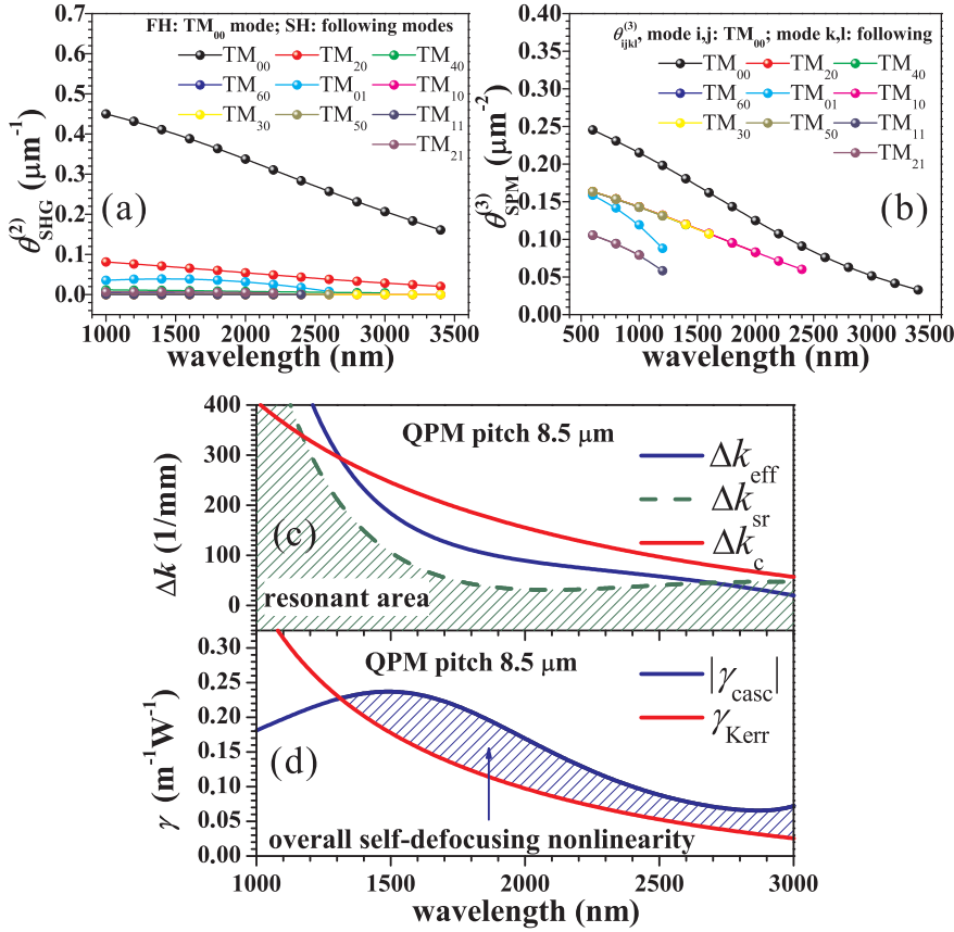
Fig. 4.13: (a) mode overlap integrals in SHG processes; (b) mode overlap integrals in self/cross phase modulations; (c) phase mismatch limits for overall self-defocusing nonlinearity and for clean soliton compressions; (d) nonlinear factors of both the cascaded quadratic nonlinearity and the Kerr nonlinearity. Waveguide has \text{wd} = 4 \mu\text{m} , \text{dp} = 2 \mu\text{m} .
