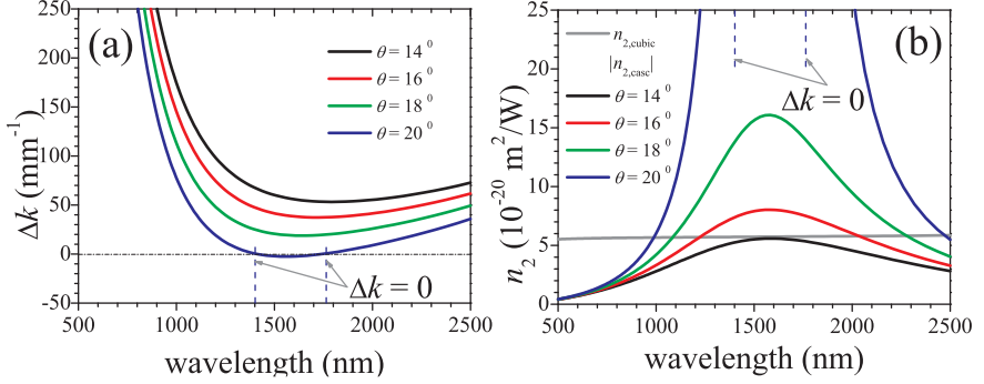
Fig. 3.1: tunability of the phase mismatch \Delta k and the cascaded quadratic nonlinearity (shown in n_{2,\text{casc}} ) as a function of FW wavelength, under different angle values. Quadratic and cubic susceptibilities used are d_{22} = 2.2 (pm/V), d_{31} = -0.16 (pm/V), \bar{\chi}_{o;ooo}^{(3)} = 550 (pm 2 /V 2 ) [5]. \varphi = -\frac{\pi}{2} . The Sellmeier function of the birefringence of BBO is obtained from the handbook [6].
