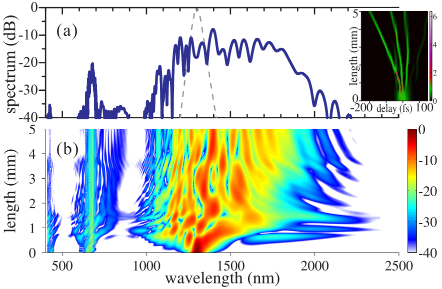
Fig. 4.10: Numerical simulation of supercontinuum generation at 1300 nm, the pump pulse has \tau_{\text{FWHM}} = 50 fs, P_{\text{avg}} = 6 \mu\text{W} , E = 6 nJ, L_{\text{D}}(\lambda = 1300\text{nm}) = 4.63 mm, L_{\text{N}} = 0.97 mm, \gamma_{\text{casc}} = -47.4 (km \cdot W) ^{-1} , \gamma_{\text{Kerr}} = 38.8 (km \cdot W) ^{-1} . f_{\text{R}} = 55\% , material dispersion of the substrate CLN is also taken into consideration; (a) supercontinuum generation at the output; (b) pulse spectral evolution during the propagation; inset in (a) pulse temporal evolution during the propagation.
